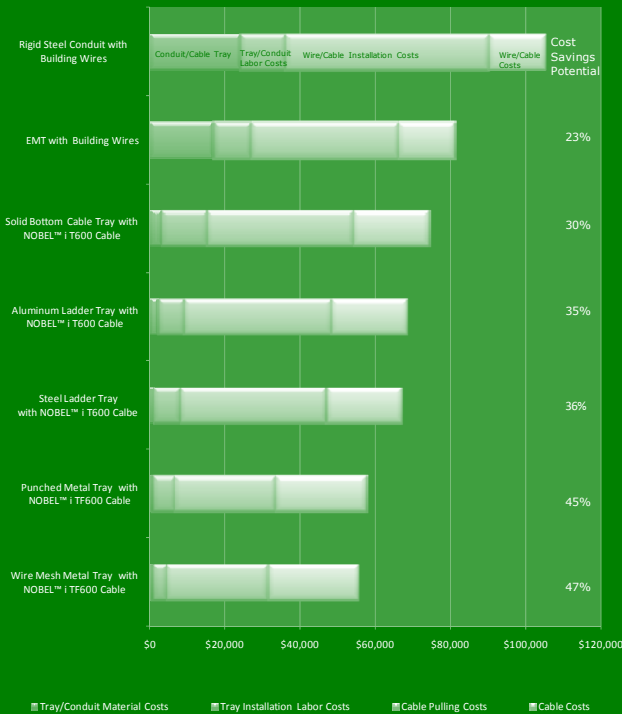
Cost Comparison of Tray and Conduit Installations
